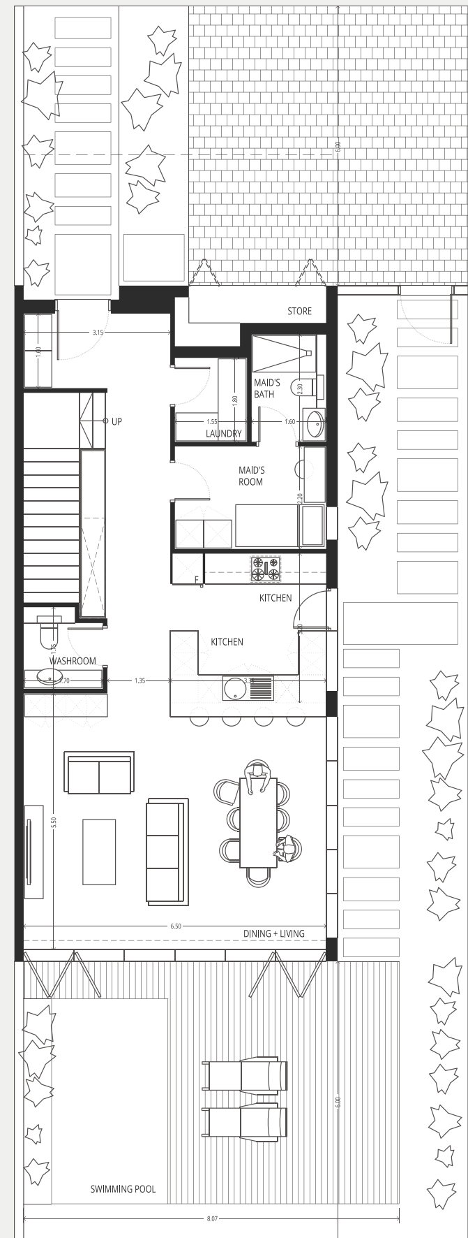
GROUND FLOOR
